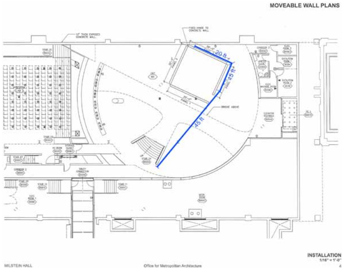
Figure 1. Common path of egress travel shown superimposed over "moveable wall plans" provided by the building architects on Dec. 10, 2010 exceeds 75 feet (email from Kim Cleveland of Accufab to Ziad Shehab of OMA Architects; blue lines and dimensions added by J. Ochshorn)
