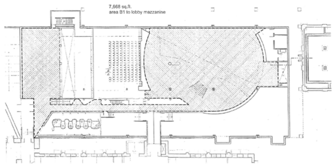
Figure 6 Plans show mezzanine as though it is within the combined crit room, auditorium, and the corridor connecting them.
