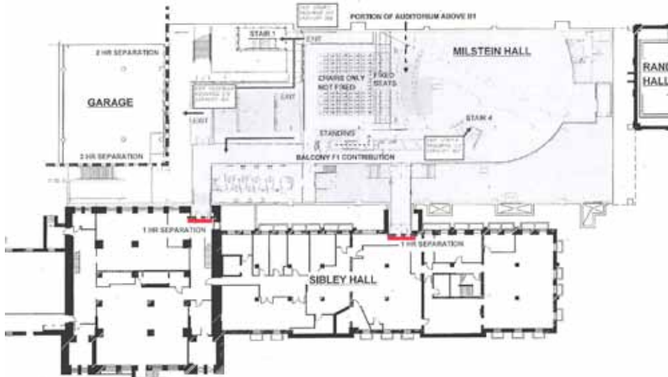
Figure 3. Fire separation shown separating the basement of Sibley from Milstein Hall (red lines have been added by J. Ochshorn to match what appeared in the original colored drawings, prepared by KHA Architects, dated 5/5/09).
