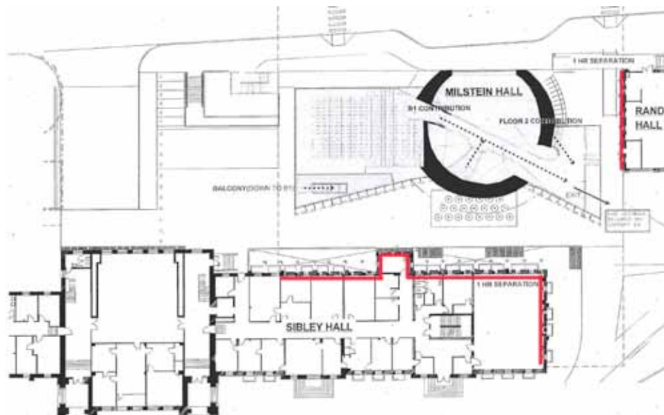
Figure 4. Fire separation at the ground level of Milstein Hall (red lines have been added by J. Ochshorn to match what appeared in the original colored drawings, prepared by KHA Architects, dated 5/5/09).
